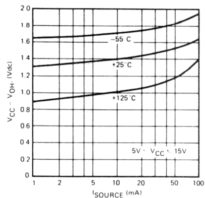
Figure 8. High Output Voltage
