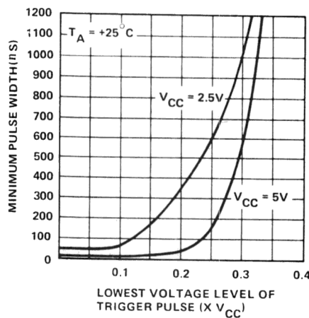
Figure 4. Minimum Pulse-Width Required for Triggering
