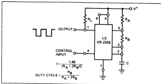
Figure 15. Astable (Free-Running) Circuit
