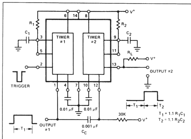
Figure 21. Sequential Timing
