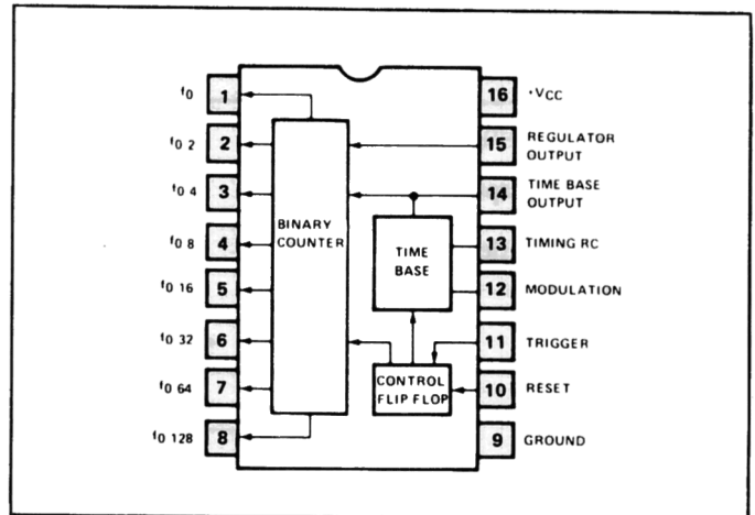
Figure 7. Functional Block Diagram of XR-2240 Timer/Counter.
