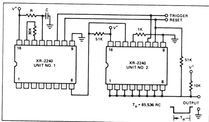
Figure 19. Cascaded Operation for Long Delay Generation
