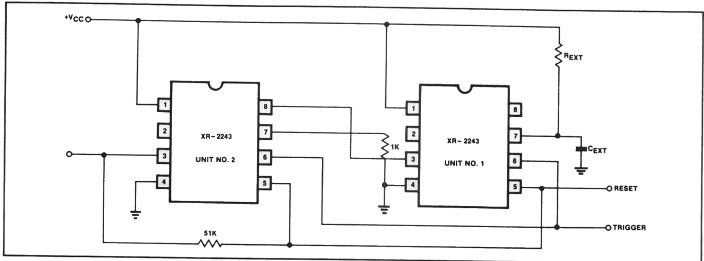
Figure 5: Cascaded Operation of Two XR-2243 Timer Circuits
