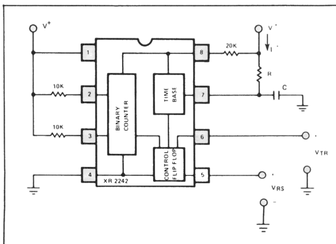
Figure 3. Generalized Test Circuit
