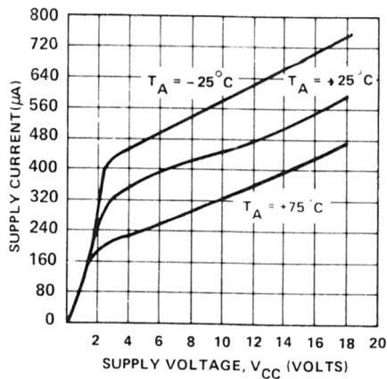
Figure 3. Total Supply Current as a Function of Supply Voltage
