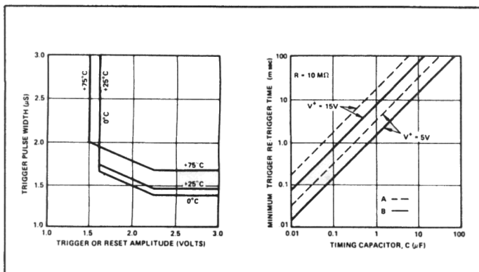
Figure 9. Minimum Trigger and Re-trigger Pulse Widths at Pins 5 and 6
