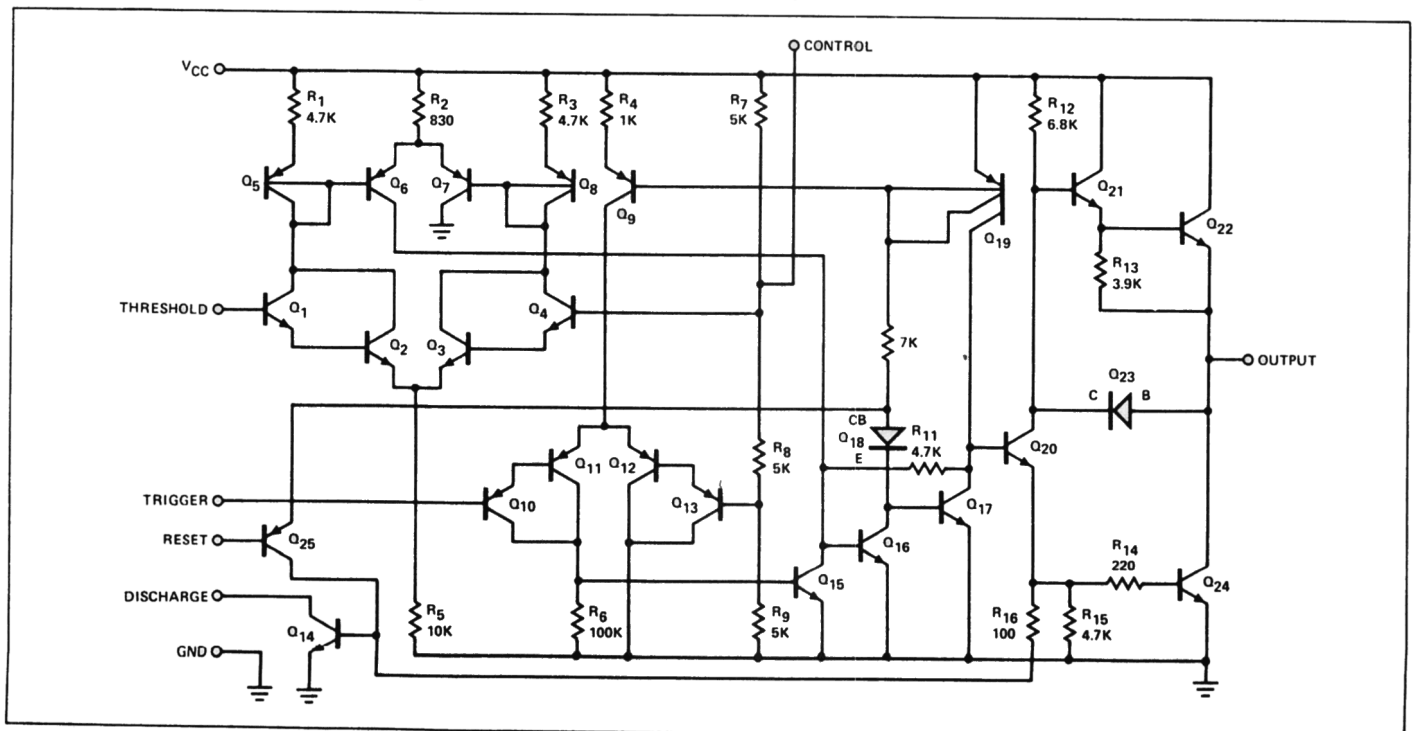
Figure 18. Circuit Schematic - 1/2 of XR-2256
