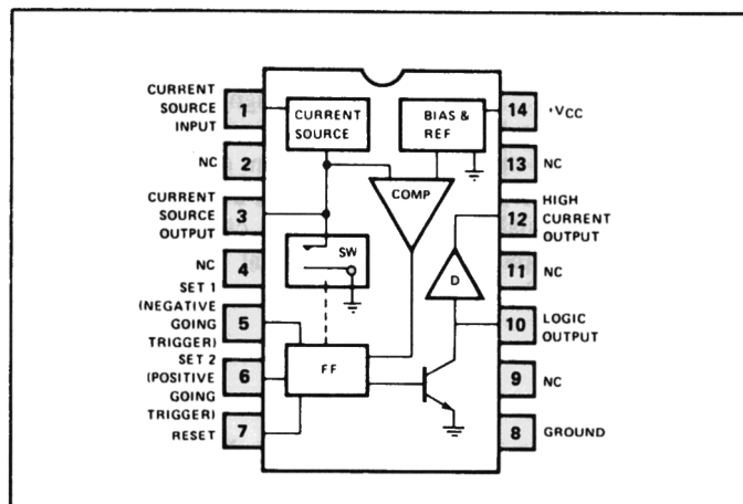
Figure 1. Functional Diagram of XR-320 Monolithic Timing Circuit.
