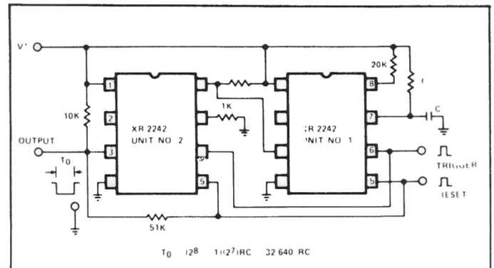
Figure 13. Cascaded Operation of Two XR-2242 Timer Circuits.
