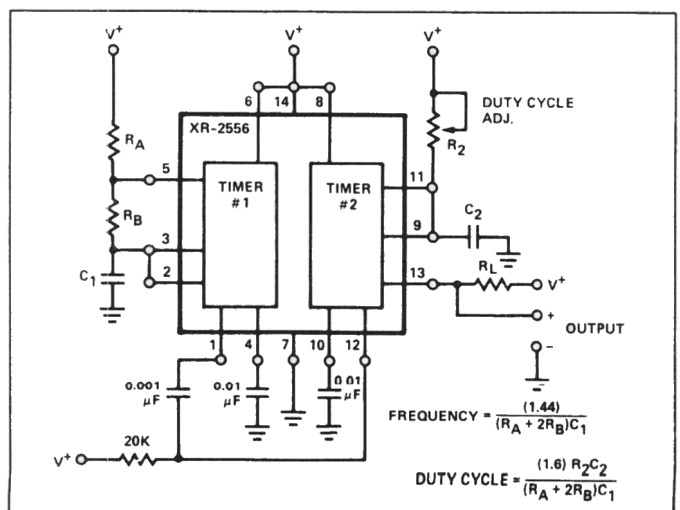
Figure 26. Fixed Frequency Oscillator With Variable Duty Cycle
