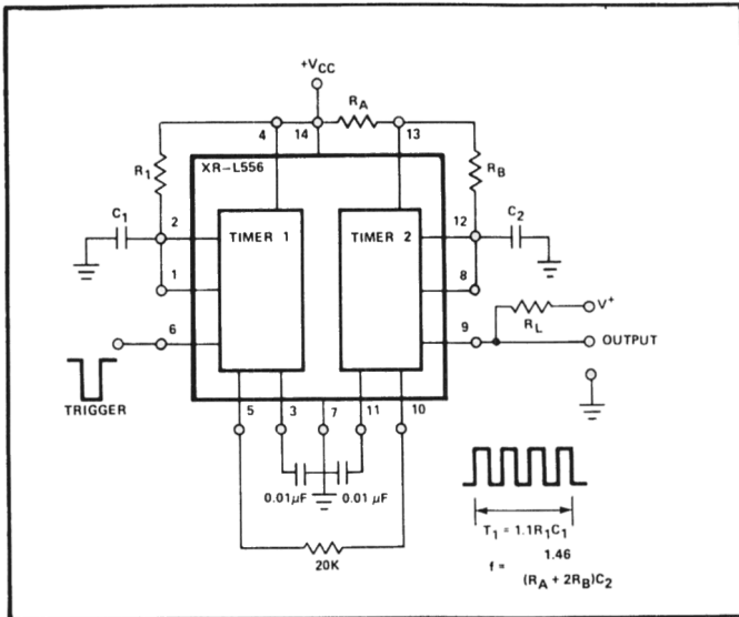
Figure 17. Keyed Oscillator
