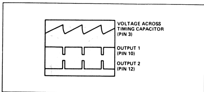
Figure 8. Waveforms for Self-Triggered Operation
