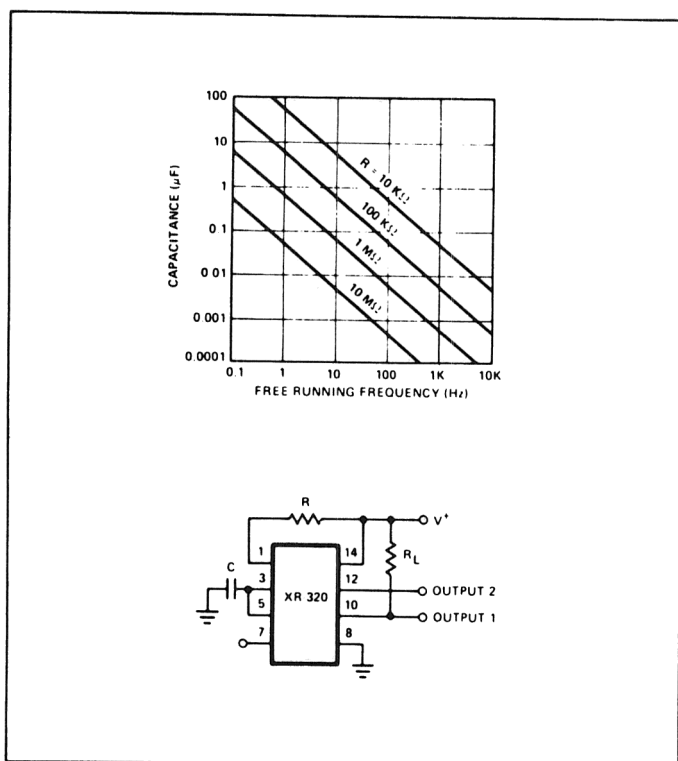
Figure 7. Free-Running Operation
