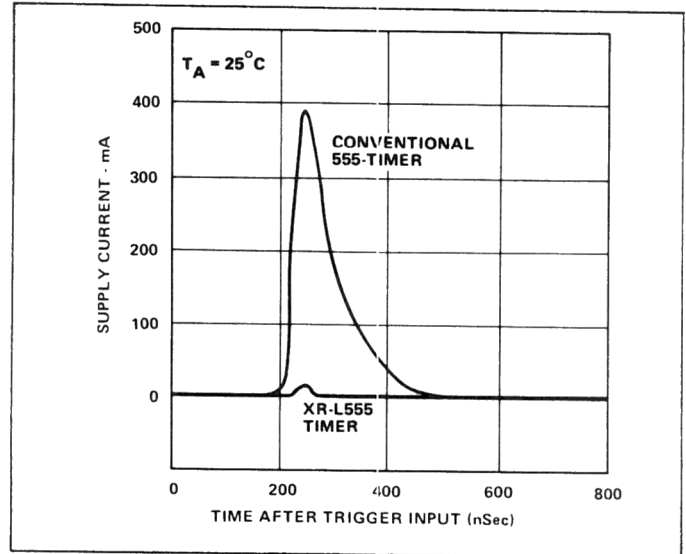
Figure 12. Comparison of Supply Current Transient of Conventional 555-Timer with XR-L555 Micropower Timer
