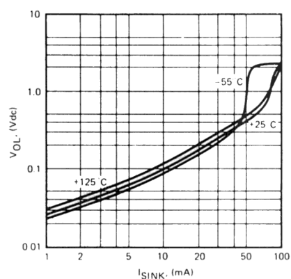
Figure 11. Low Output Voltage V_{CC} = 15 \text{ V}_{dc}
