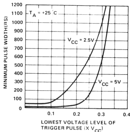
Figure 4. Minimum Pulse-Width Required for Triggering
