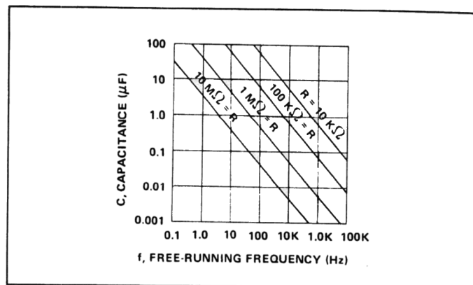
Figure 14. Free Running Frequency as a Function of External Timing Components (Note: R = R_A + 2R_B )
