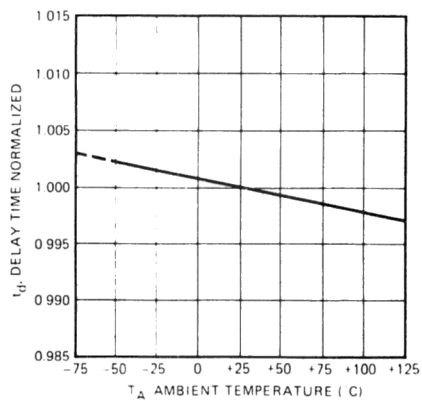
Figure 13. Delay Time vs. Temperature
