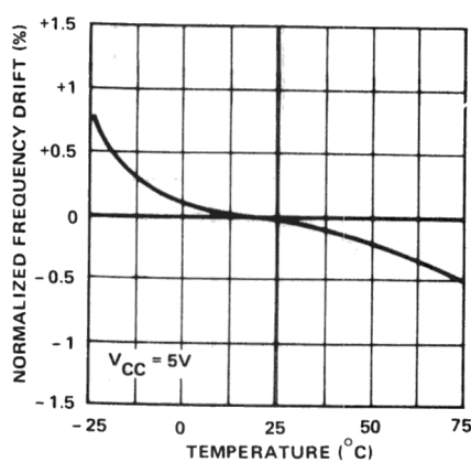
Figure 10. Typical Frequency Stability as a Function of Temperature ( R_A = R_B = 10K\Omega , C = 0.1\mu F )
