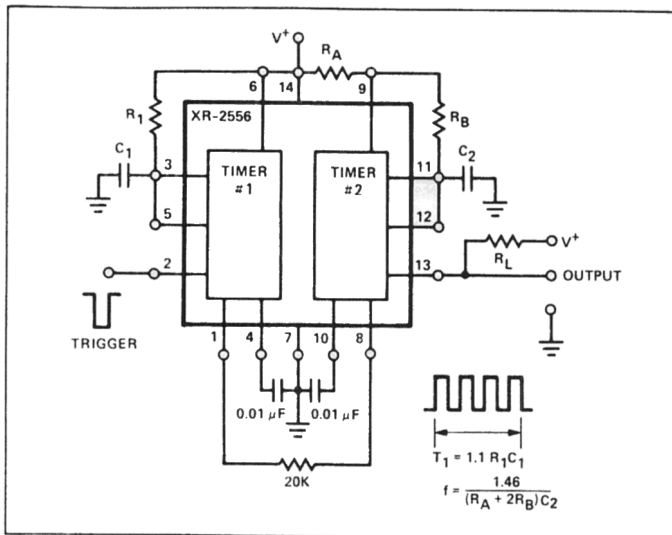
Figure 22. Keyed Oscillator
