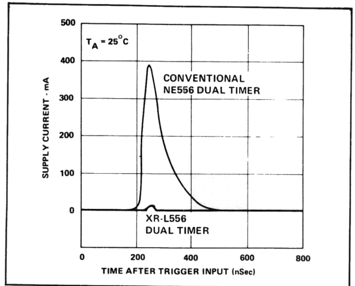
Figure 12. Comparison of Supply Current Transient of Conventional NE556 Dual Timer with XR-L556 Micropower Dual Timer
