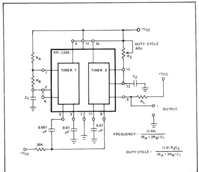
Figure 19. Micropower Oscillator with Fixed Frequency and Variable Duty-Cycle
