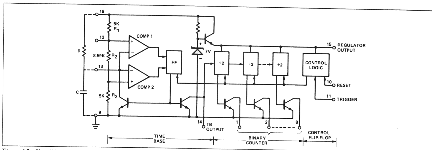
Figure 15. Simplified Circuit Diagram of XR-2240
