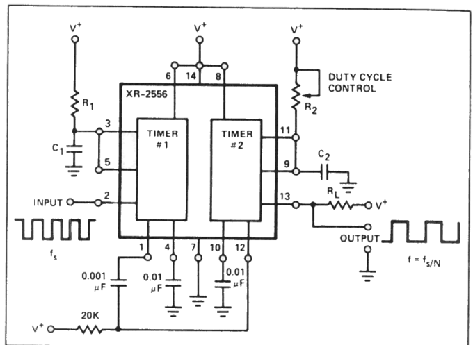
Figure 24. Frequency Divider and Pulse-Shaper
