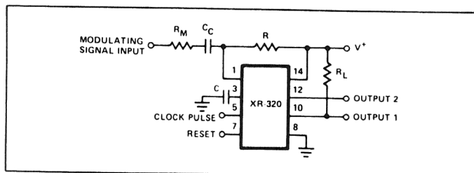
Figure 9. Circuit Connection for Pulse-Width Modulation
