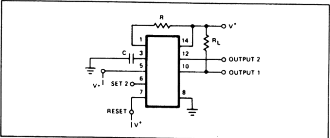
Figure 3. Monostable Operation, Positive Trigger
