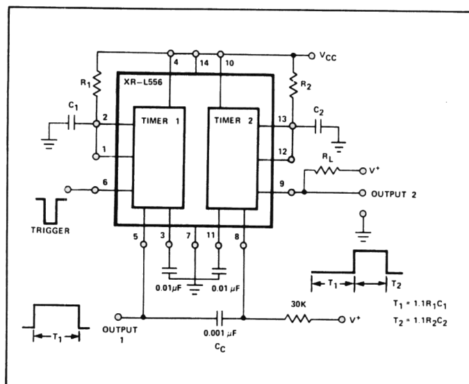
Figure 16. Sequential Timing
