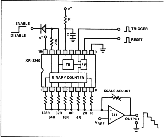
Figure 26. Staircase Generator
