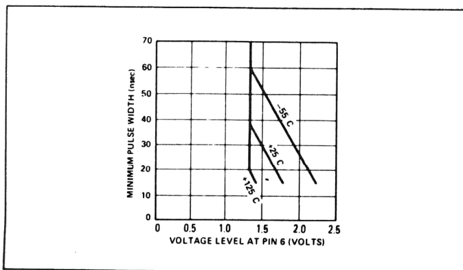
Figure 12. Minimum Pulse Width for Triggering at Pin 6
