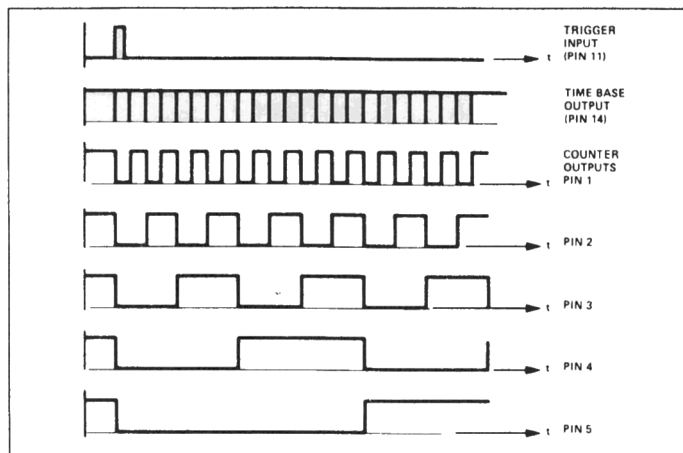
Figure 5. Timing Diagram of Output Waveforms
