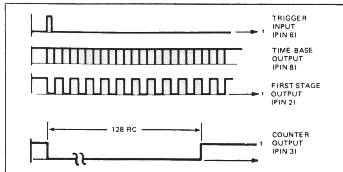
Figure 7. Timing Diagram of Output Waveforms
