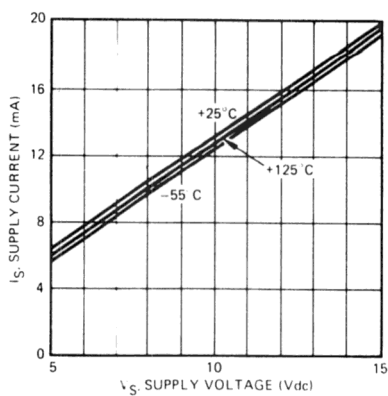
Figure 7. Supply Current (Both Timer Sections)
