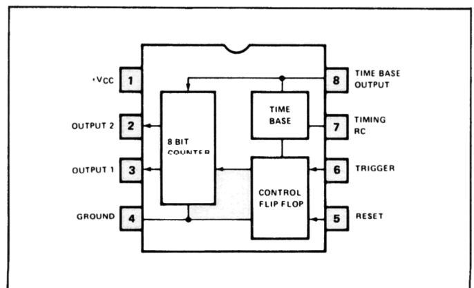
Figure 8. Package Diagram of XR-2242 Long-Range Timer.
