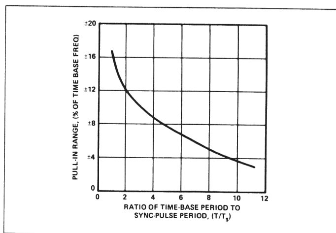
Figure 17. Typical Pull-In Range for Harmonic Synchronization
