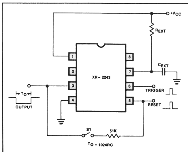
Figure 3: Typical Operation Diagram
