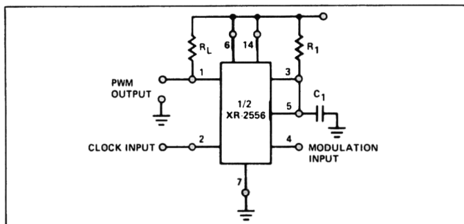
Figure 27. Pulse-Width Modulation
