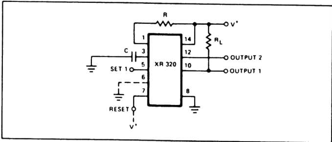
Figure 2. Monostable Operation, Negative Trigger
