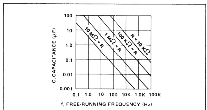
Figure 14. Free Running Frequency as a Function of External Timing Components (Note: R = R_A + 2R_B )
