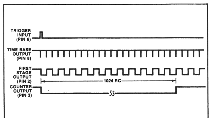
Figure 4: Timing Diagram of Output Waveforms
