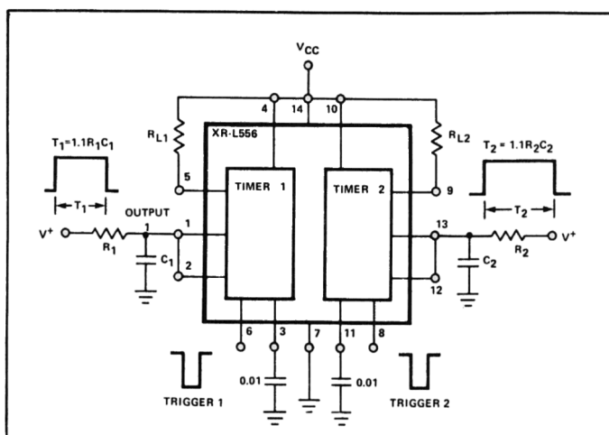
Figure 15. Generation of Two Independent Time Delays
