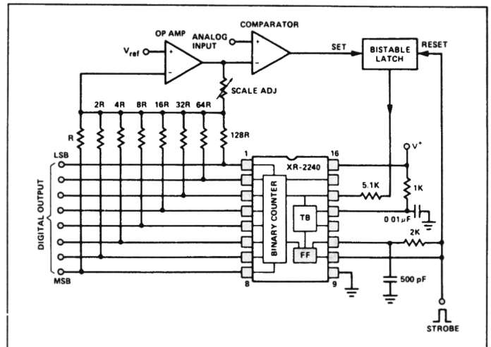
Figure 28. Analog-To-Digital Converter
