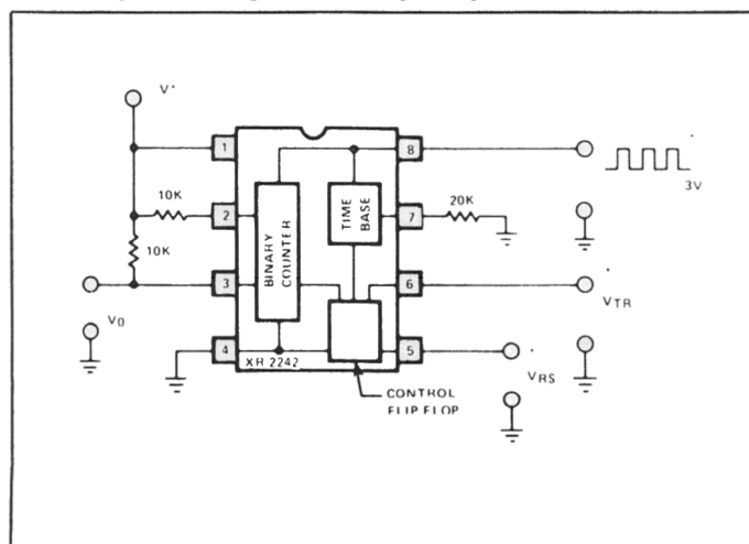
Figure 4. Test for Counter Section
