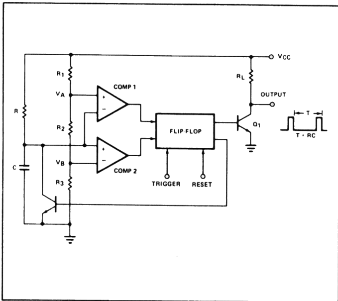
Figure 4. Simplified Schematic of a Time-Base Oscillator Circuit
