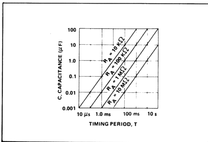
Figure 13. Timing Period, T, as a Function of External R-C Network
