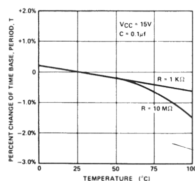
Figure 14. Temperature Drift of Time-Base Period, T
