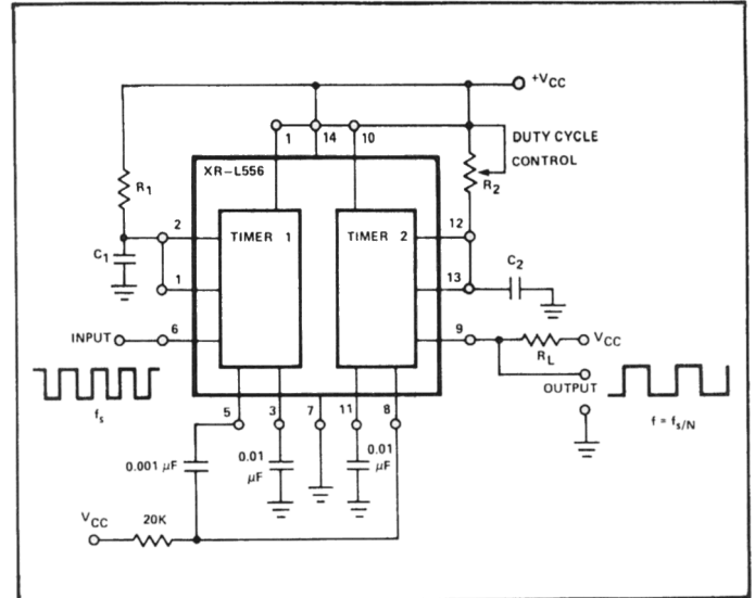
Figure 18. Frequency Divider and Pulse-Shaper
