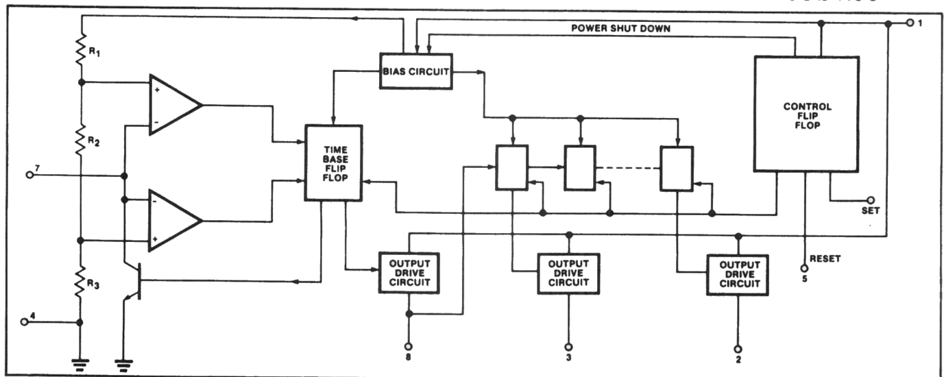
Figure 2: Simplified Circuit Schematic
