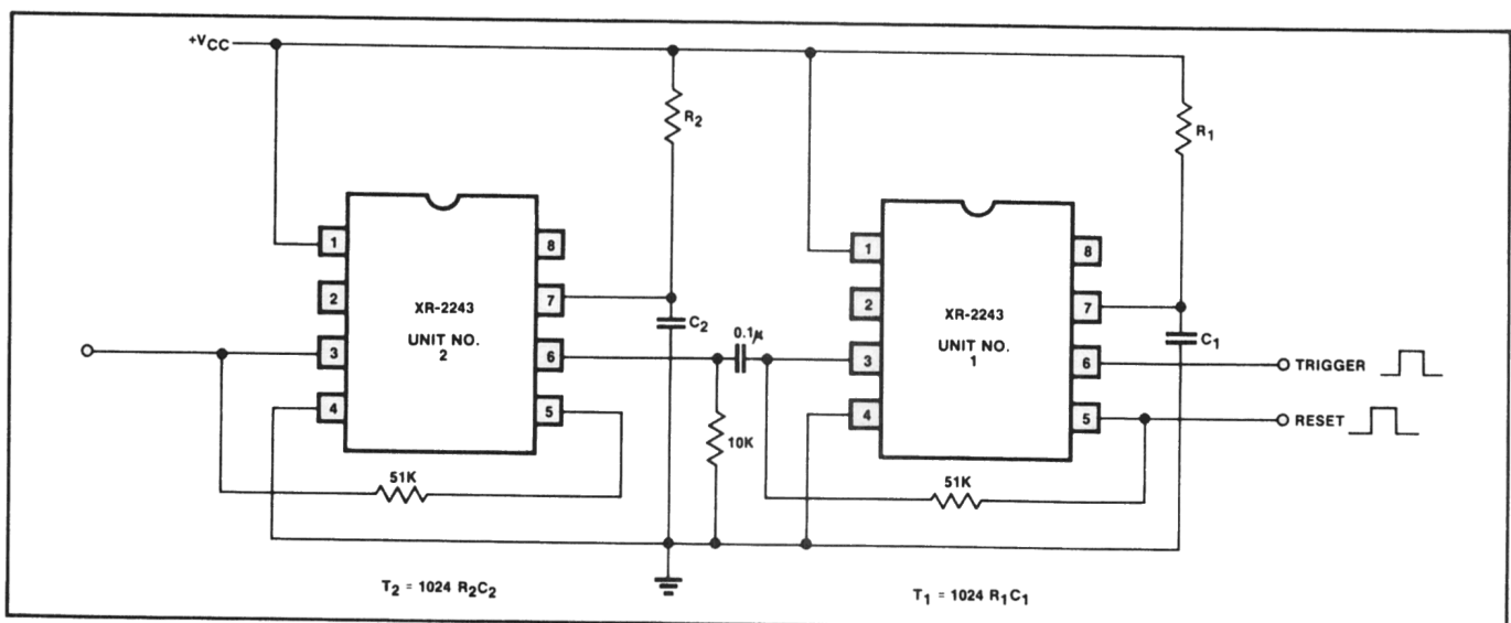
Figure 6: Sequential Timing Using XR-2243 Timer Circuits
