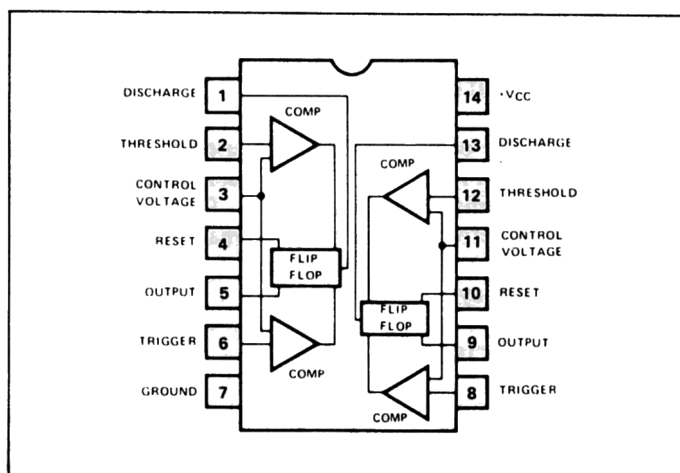
Figure 3. Functional Diagram of XR-556 Dual Timer.
