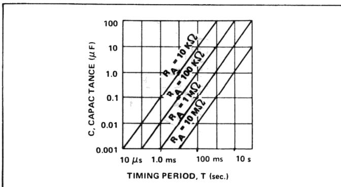
Figure 13. Timing Period, T , as a Function of External R-C Network
