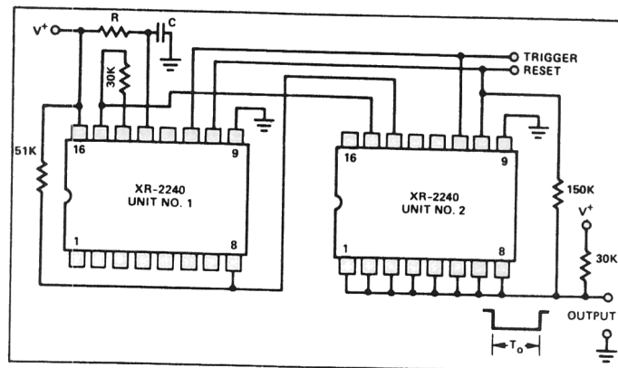
Figure 20. Low-Power Operation of Cascaded Timers
