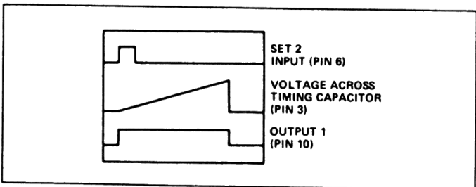
Figure 5. Waveforms for Positive-Going Trigger
