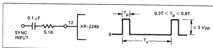
Figure 16. Operation with External Sync Signal.
