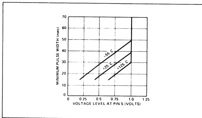
Figure 11. Minimum Pulse Width for Triggering at Pin 5
