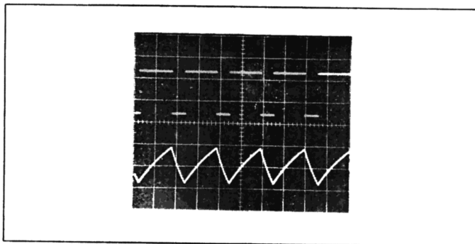
Figure 16. Astable Waveforms
