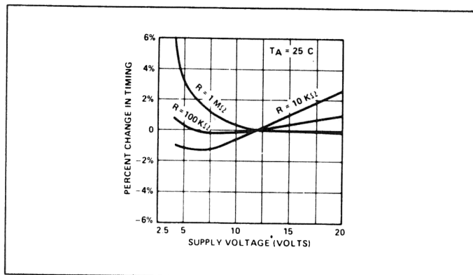
Figure 10. Change in Timing vs. Supply Voltage
