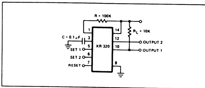
Figure 1. Test Circuit
