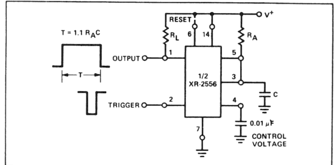
Figure 3. Monostable (One-Shot) Circuit
