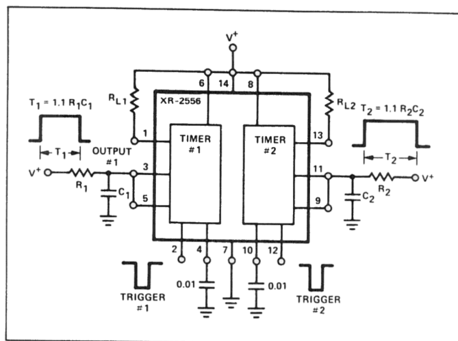
Figure 20. Generation of Two Independent Time Delays
