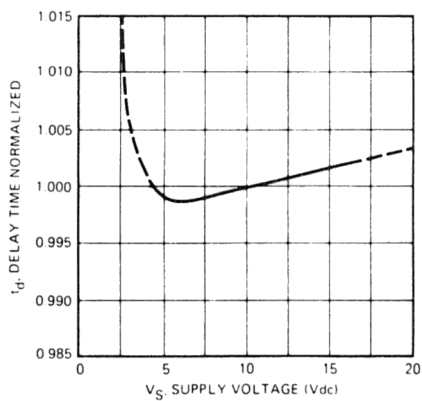
Figure 12. Delay Time vs. Supply Voltage
