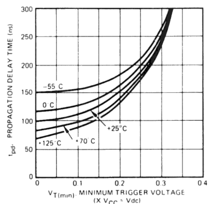
Figure 14. Propagation Delay vs. Trigger Voltage
