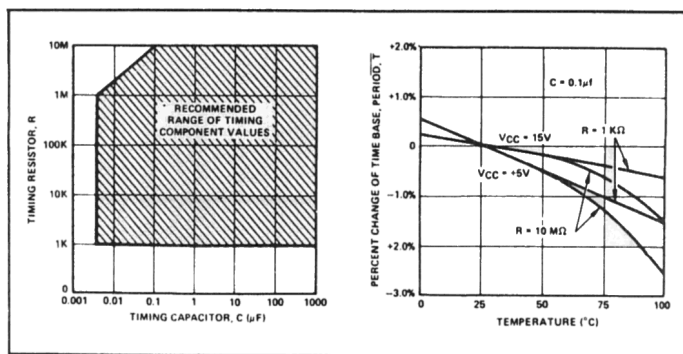
Figure 5. Recommended Range of Timing Component Values
