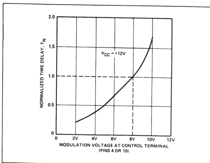
Figure 19. Normalized Time Delay vs. Modulation Voltage
