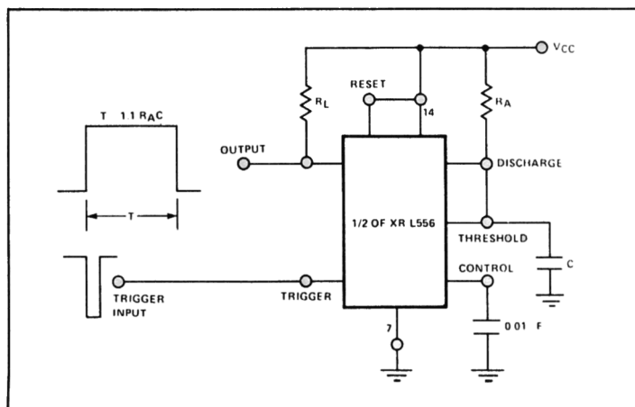
Figure 1. Monostable (One-Shot) Circuit
